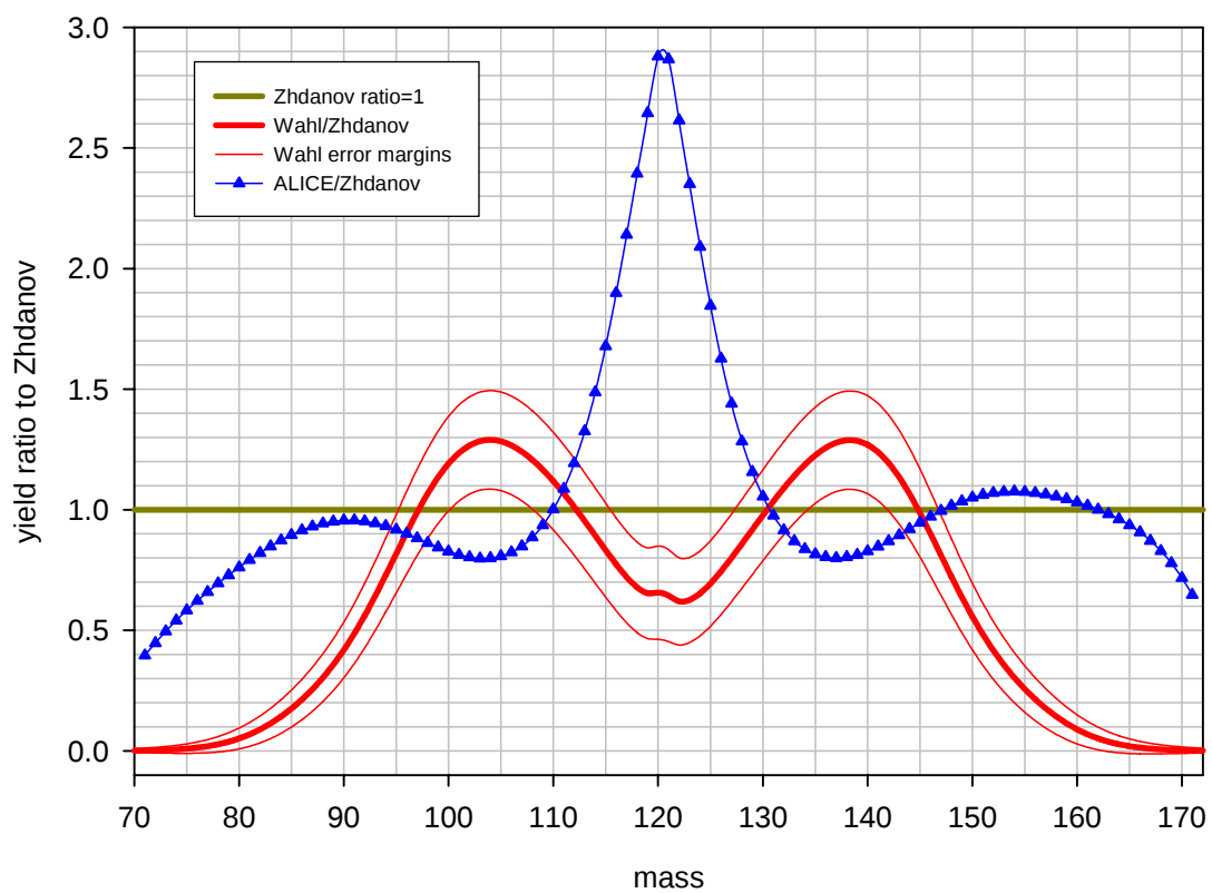
Benchmark B: ^{241}\text{Am} at 13 MeV, pre-neutron emission yield ratio to Zhdanov's data
